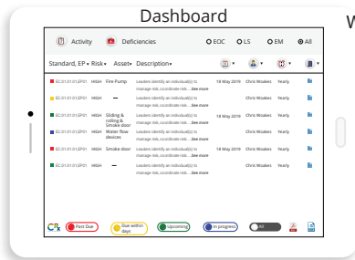
Risk Management
